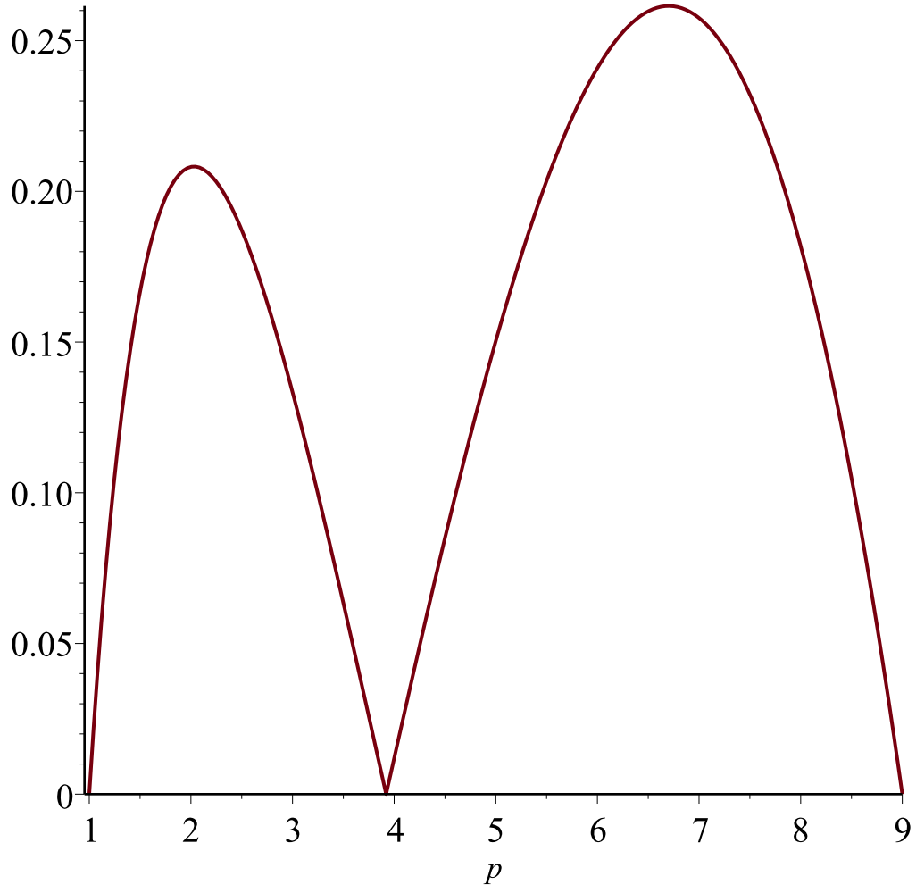
Error Function of f11 for epsilon=-0.1
