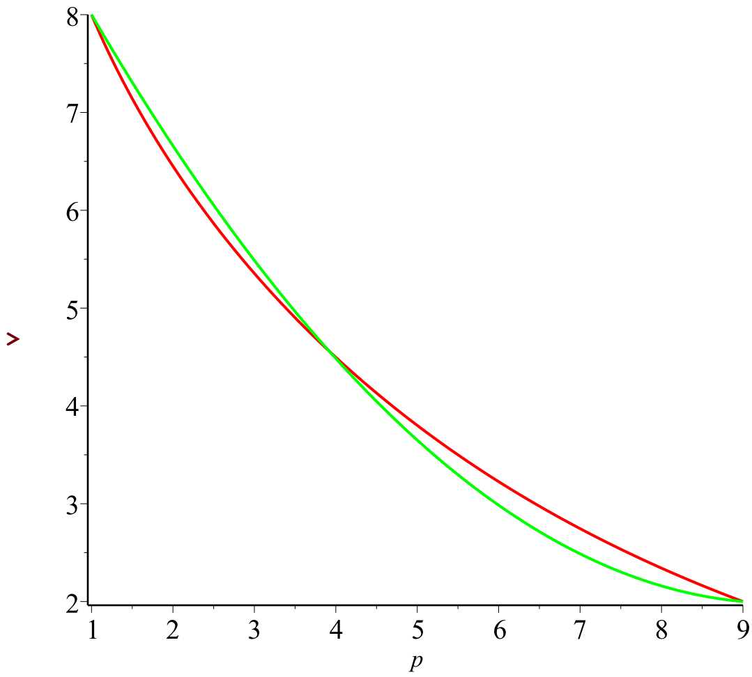
f11 compare with q(p) when epsilon=-0.1
