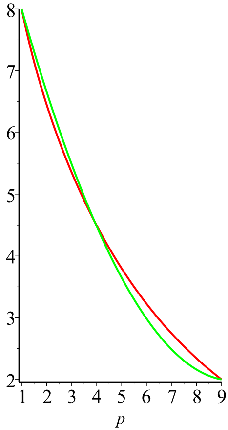
f11 compare with q(p) when epsilon=-0.1
